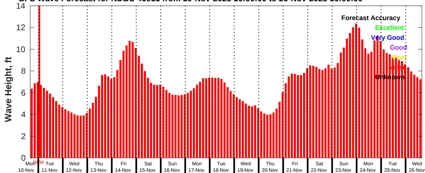
GFS Wave Forecast for NDBC 46011 from 10-Nov-2025 16:00:00 to 26-Nov-2025 16:00:00
