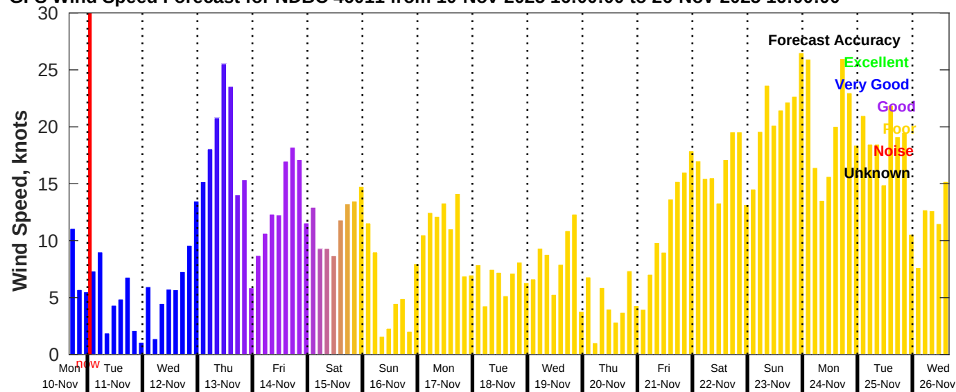
GFS Wind Speed Forecast for NDBC 46011 from 10-Nov-2025 16:00:00 to 26-Nov-2025 16:00:00
