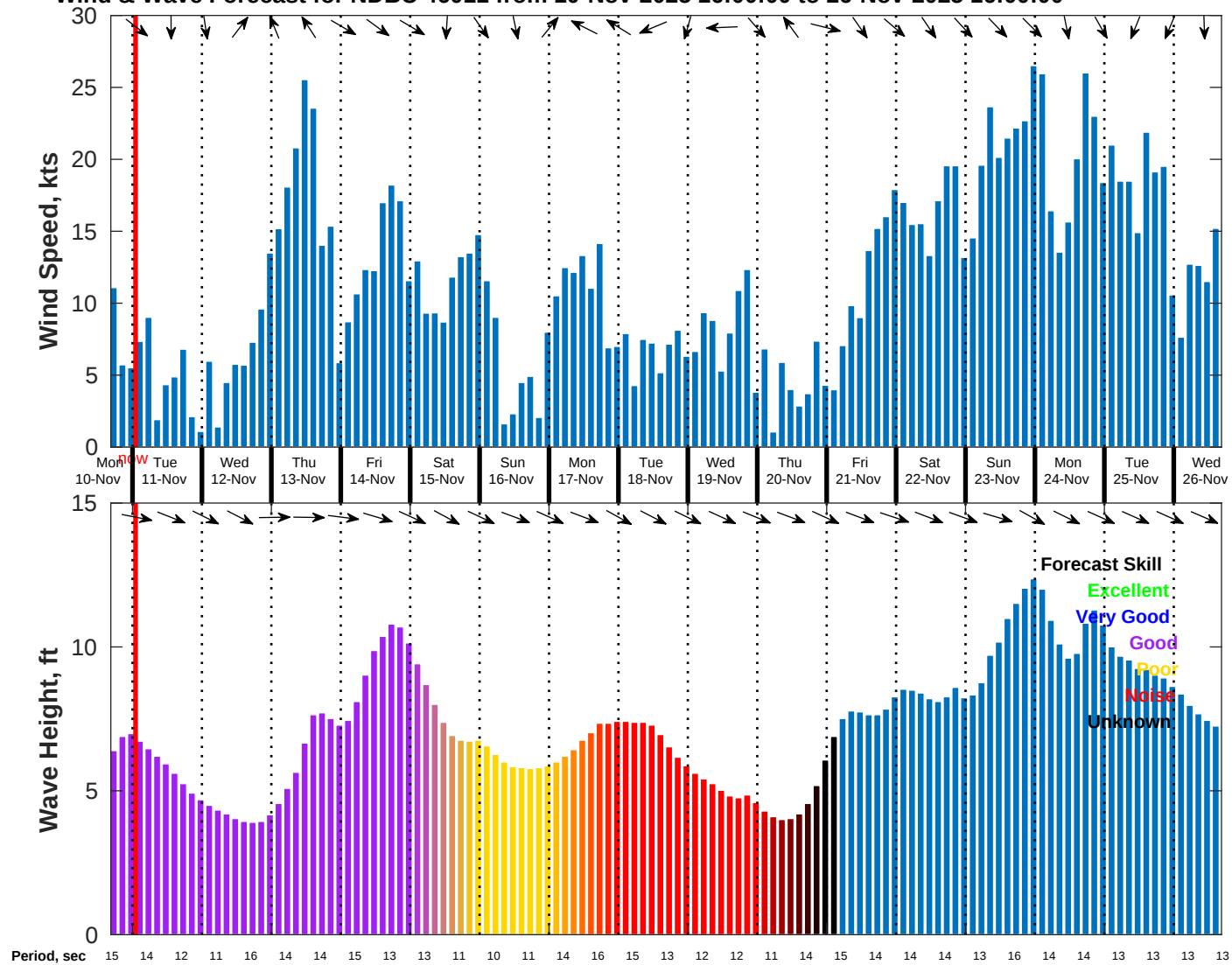
Wind & Wave Forecast for NDBC 46011 from 10-Nov-2025 16:00:00 to 26-Nov-2025 16:00:00
