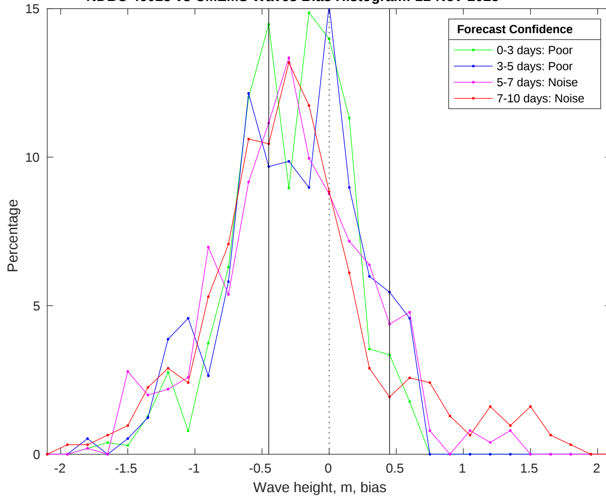
NDBC 46028 vs CMEMS Waves Bias Histogram: 11-Nov-2025
