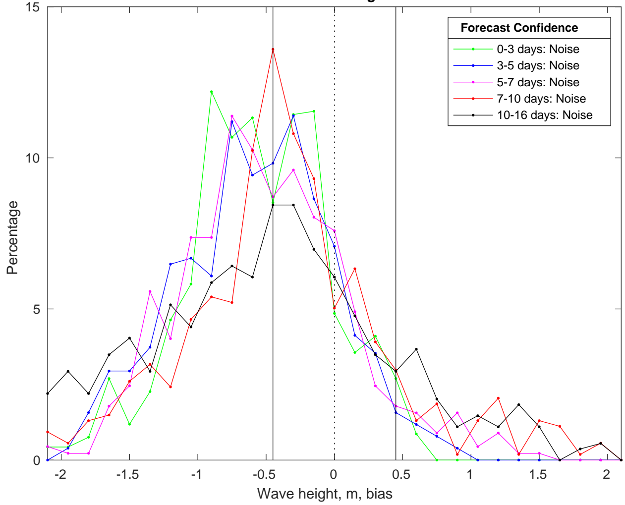
NDBC 46028 vs GFS Waves Bias Histogram: 11-Nov-2025
