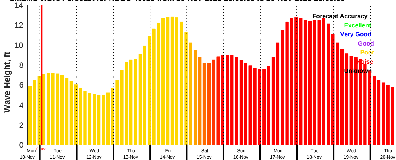
CMEMS Wave Forecast for NDBC 46028 from 10-Nov-2025 16:00:00 to 20-Nov-2025 16:00:00
