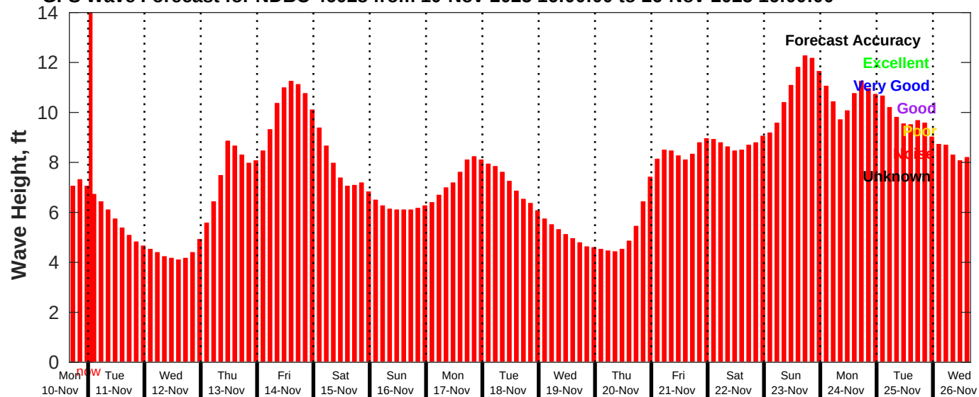
GFS Wave Forecast for NDBC 46028 from 10-Nov-2025 16:00:00 to 26-Nov-2025 16:00:00
