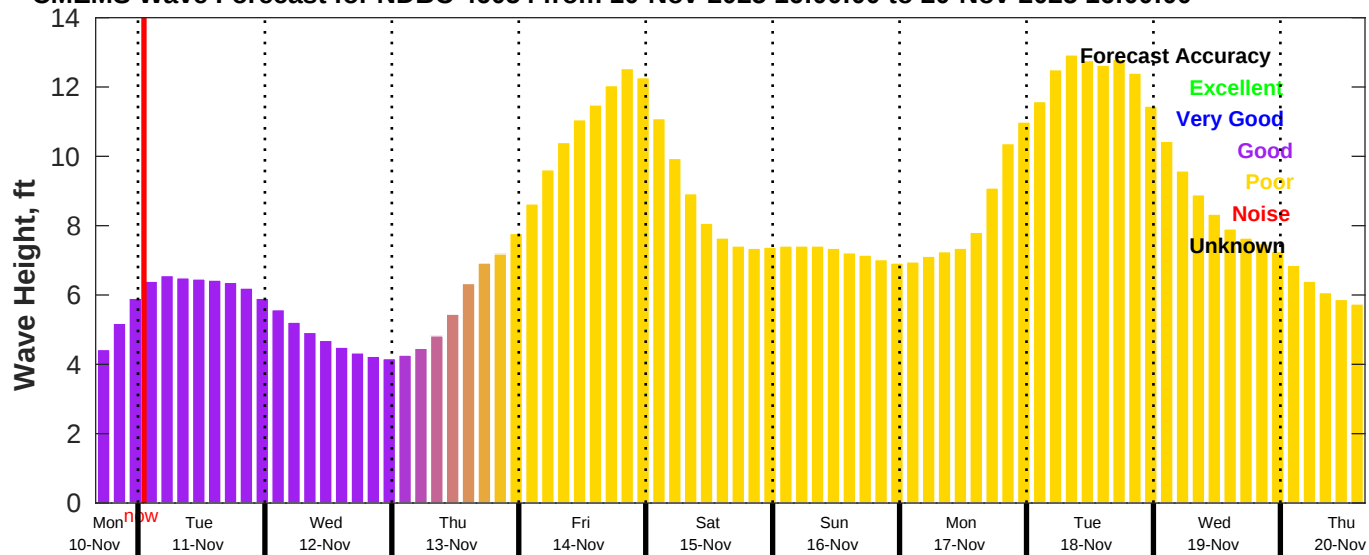
CMEMS Wave Forecast for NDBC 46054 from 10-Nov-2025 16:00:00 to 20-Nov-2025 16:00:00
