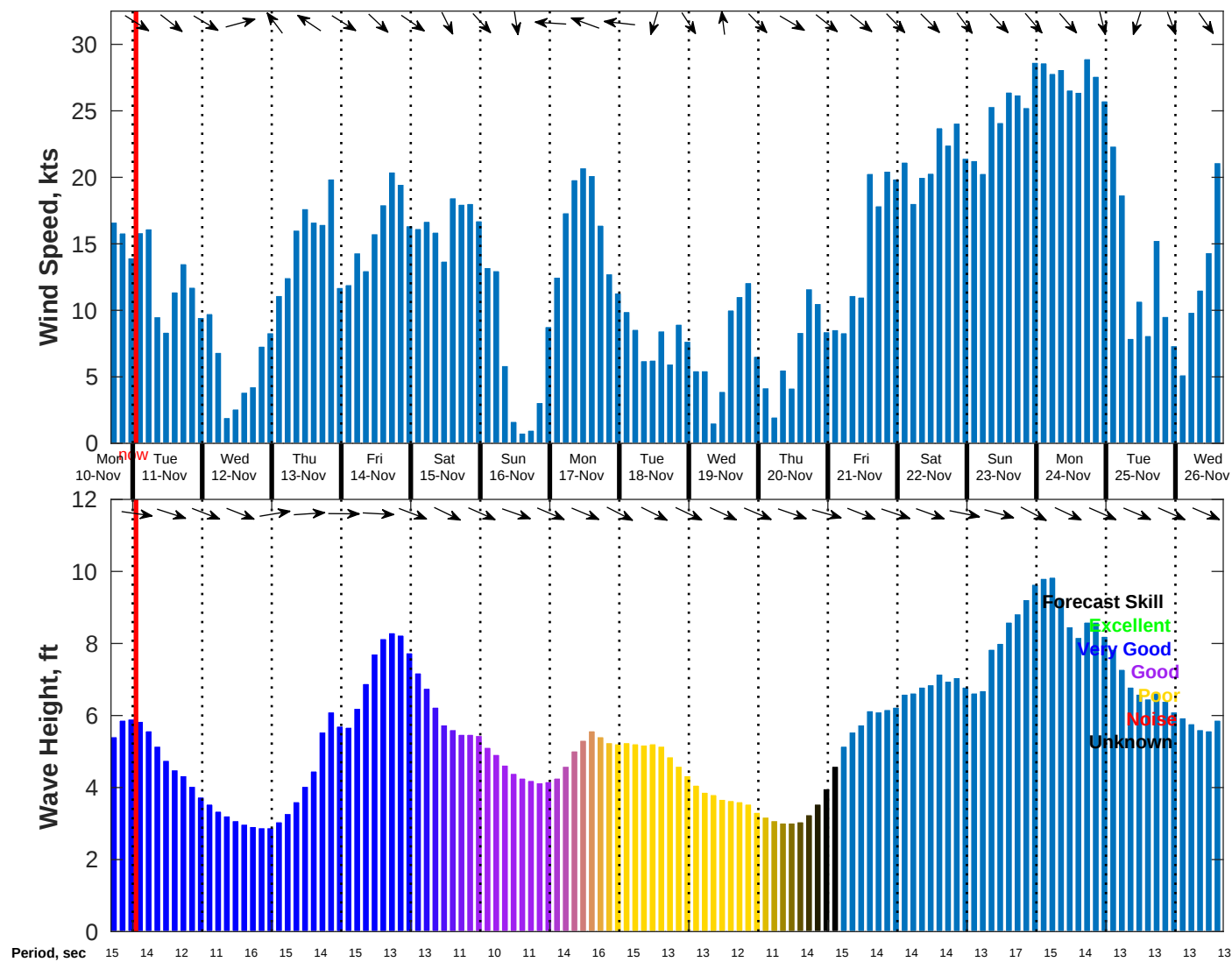
Wind & Wave Forecast for NDBC 46054 from 10-Nov-2025 16:00:00 to 26-Nov-2025 16:00:00
