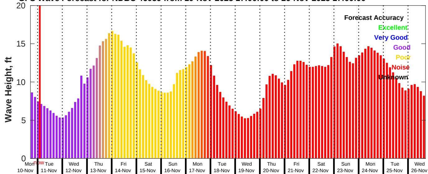
GFS Wave Forecast for NDBC 46059 from 10-Nov-2025 17:00:00 to 26-Nov-2025 17:00:00
