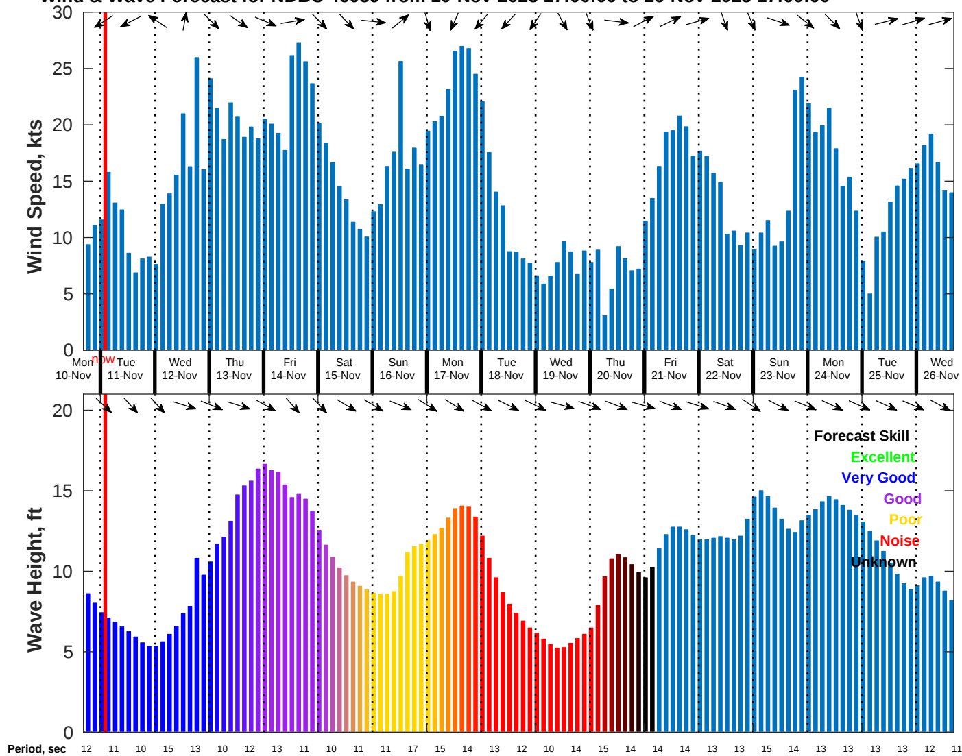
Wind & Wave Forecast for NDBC 46059 from 10-Nov-2025 17:00:00 to 26-Nov-2025 17:00:00
