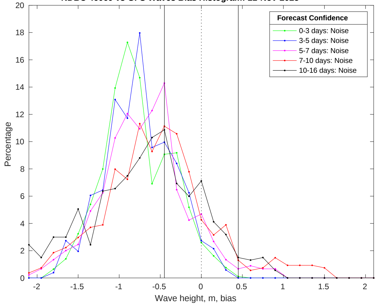
NDBC 46069 vs GFS Waves Bias Histogram: 11-Nov-2025
