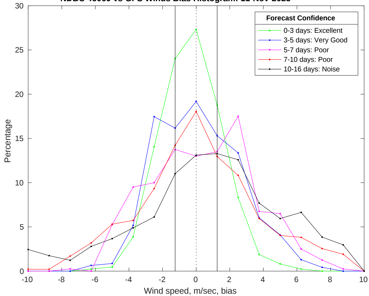
NDBC 46069 vs GFS Winds Bias Histogram: 11-Nov-2025
