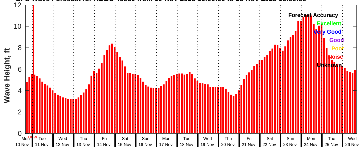
GFS Wave Forecast for NDBC 46069 from 10-Nov-2025 16:00:00 to 26-Nov-2025 16:00:00
