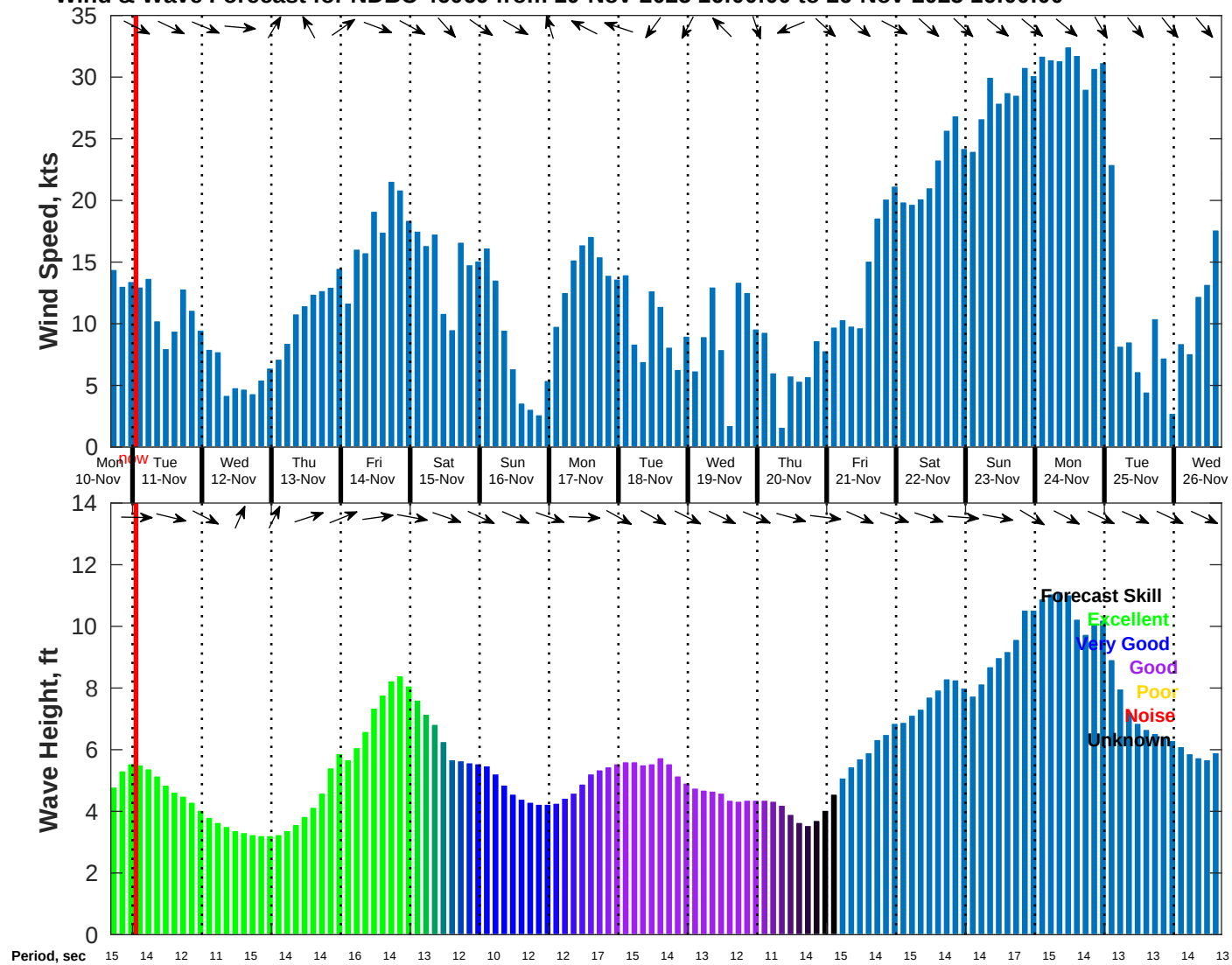
Wind & Wave Forecast for NDBC 46069 from 10-Nov-2025 16:00:00 to 26-Nov-2025 16:00:00
