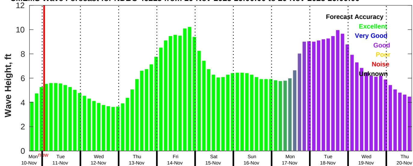
CMEMS Wave Forecast for NDBC 46215 from 10-Nov-2025 16:00:00 to 20-Nov-2025 16:00:00
