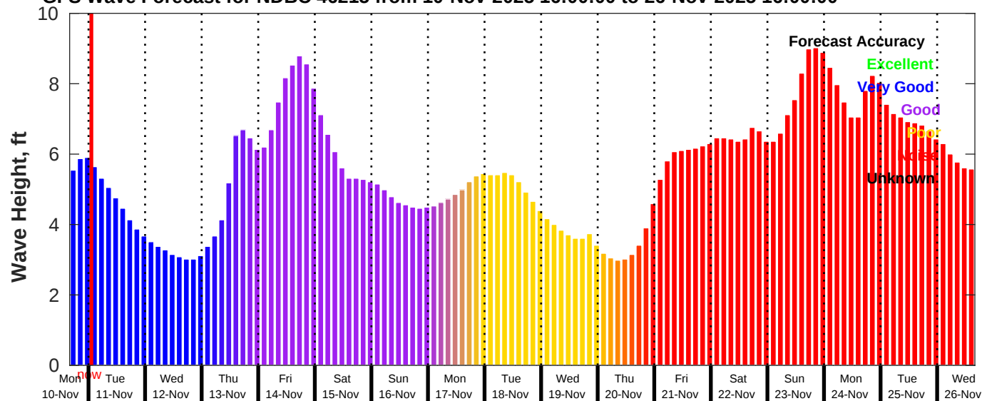
GFS Wave Forecast for NDBC 46215 from 10-Nov-2025 16:00:00 to 26-Nov-2025 16:00:00
