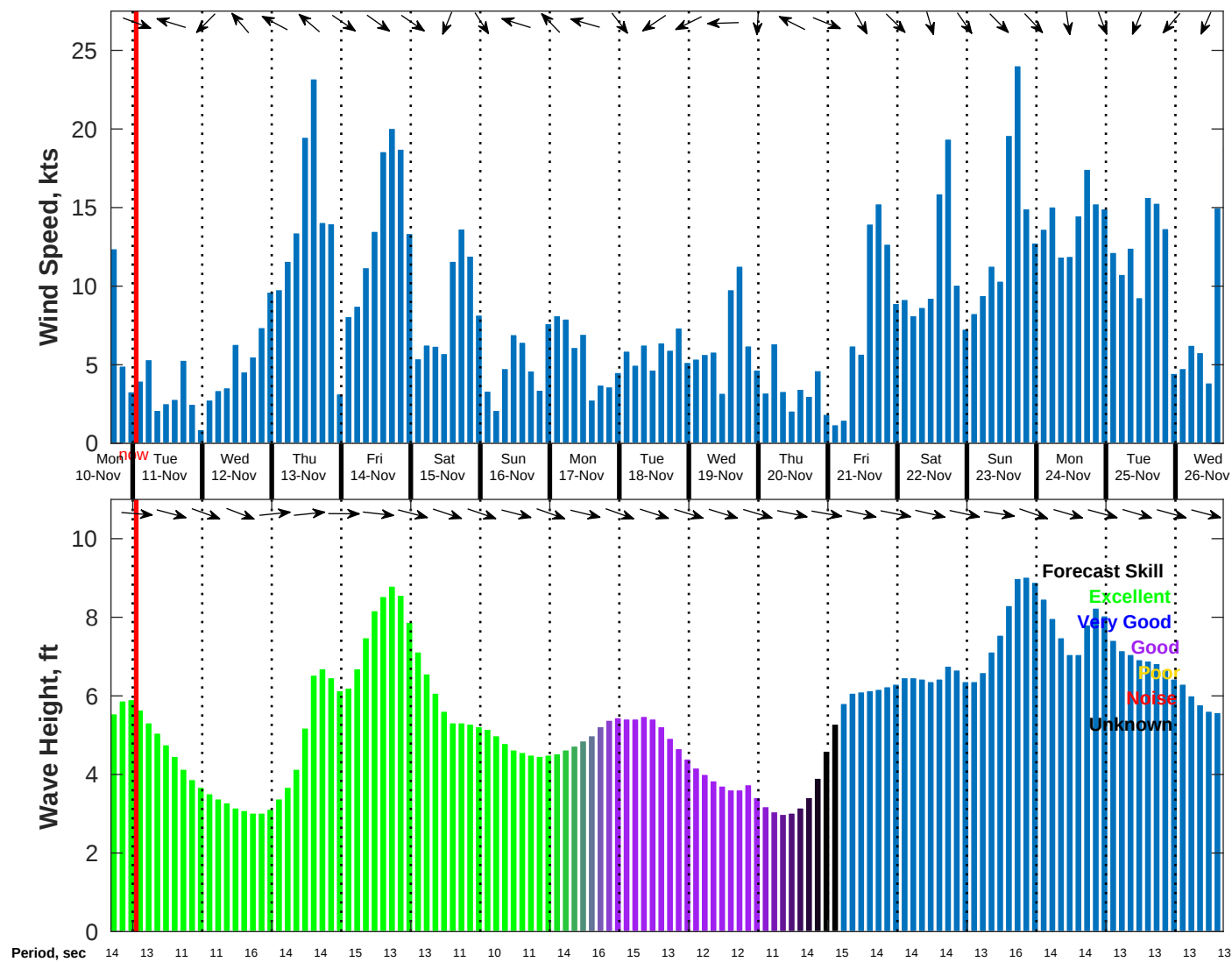
Wind & Wave Forecast for NDBC 46215 from 10-Nov-2025 16:00:00 to 26-Nov-2025 16:00:00
