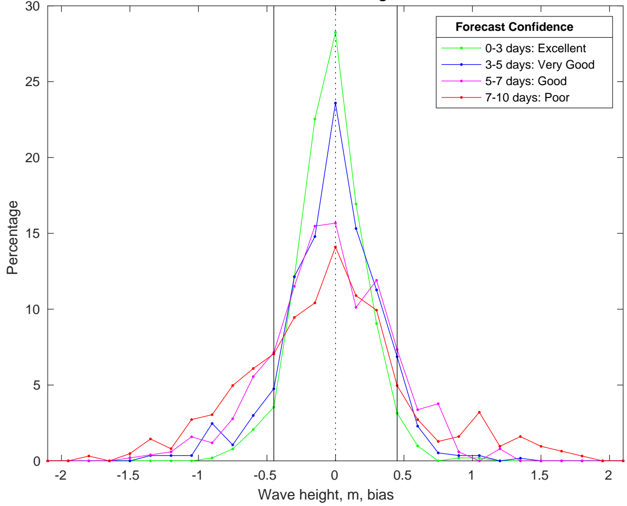
NDBC 46259 vs CMEMS Waves Bias Histogram: 11-Nov-2025
