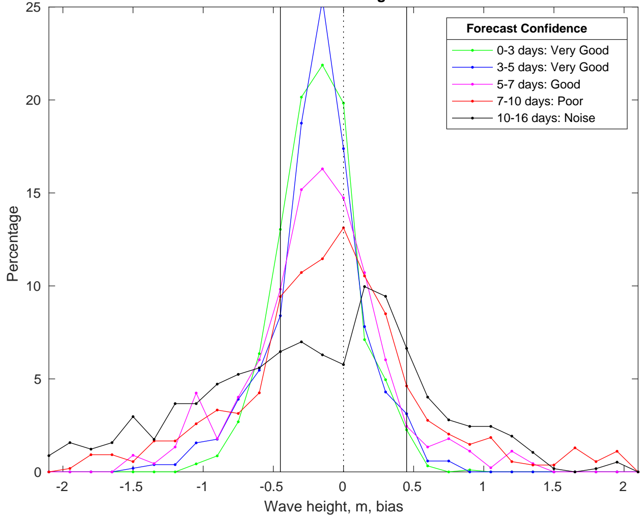
NDBC 46259 vs GFS Waves Bias Histogram: 11-Nov-2025
