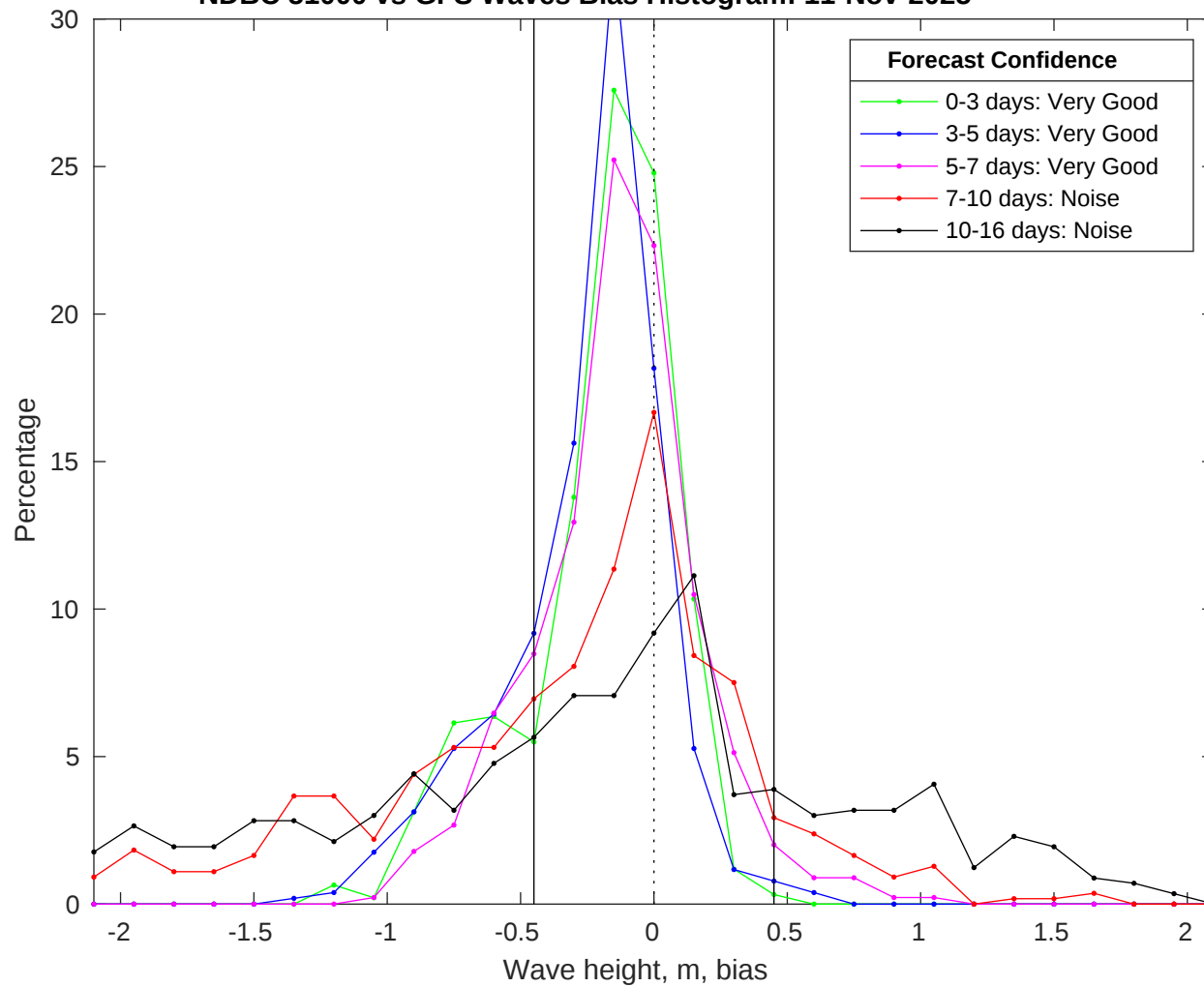
NDBC 51000 vs GFS Waves Bias Histogram: 11-Nov-2025
