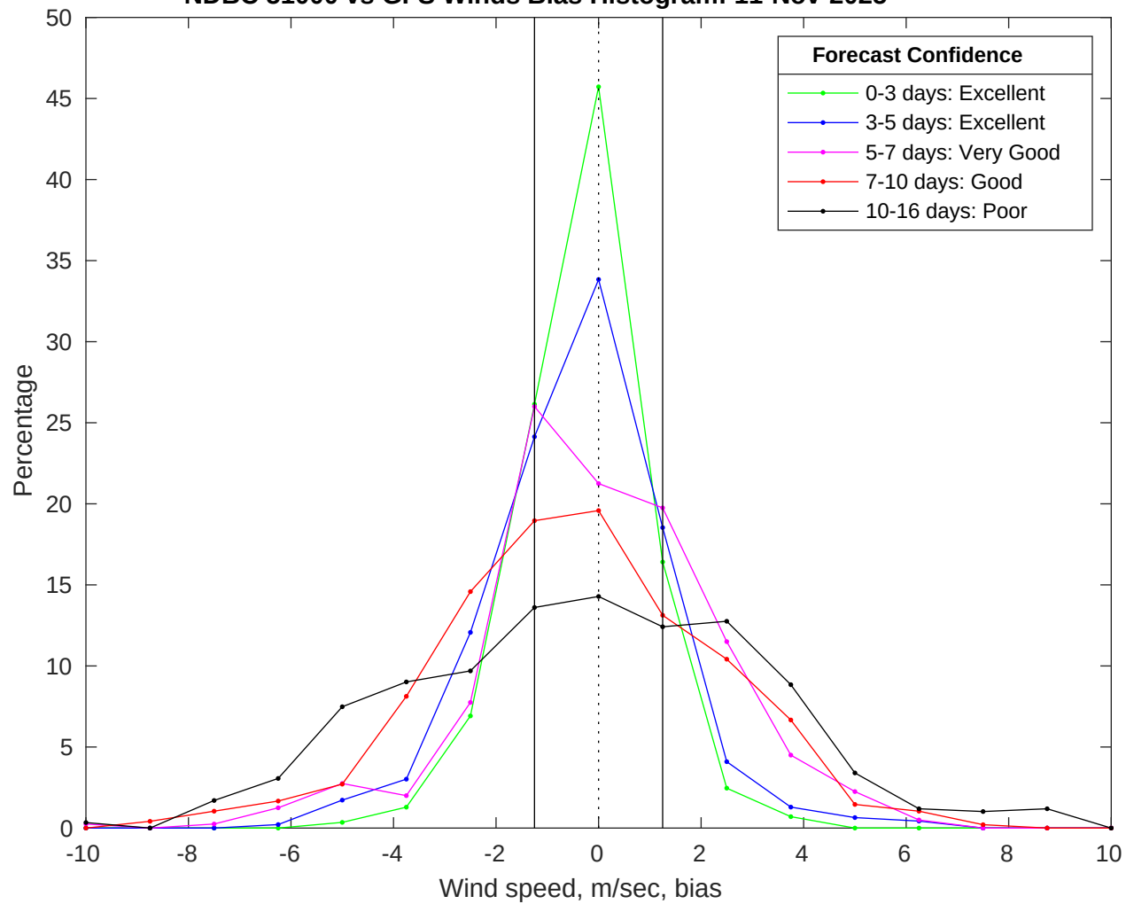
NDBC 51000 vs GFS Winds Bias Histogram: 11-Nov-2025
