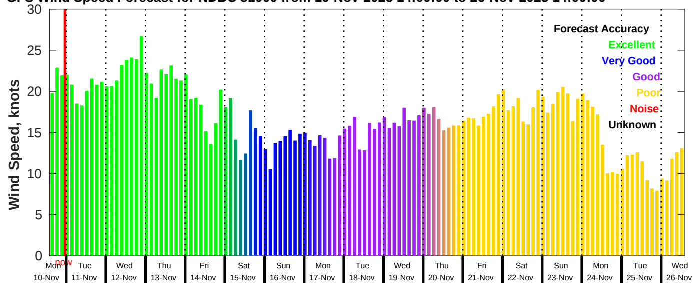
GFS Wind Speed Forecast for NDBC 51000 from 10-Nov-2025 14:00:00 to 26-Nov-2025 14:00:00
