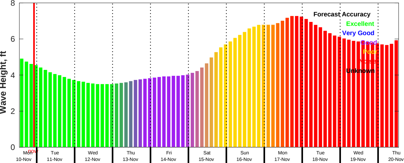
CMEMS Wave Forecast for NDBC 51209 from 10-Nov-2025 13:00:00 to 20-Nov-2025 13:00:00
