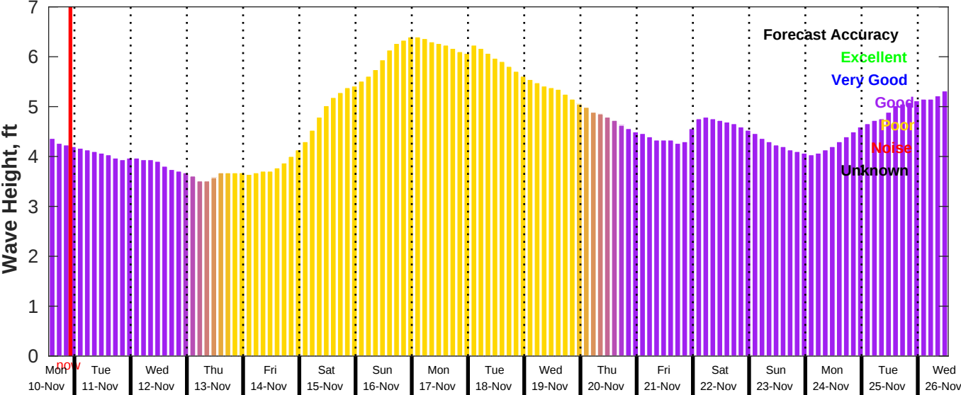
GFS Wave Forecast for NDBC 51209 from 10-Nov-2025 13:00:00 to 26-Nov-2025 13:00:00
