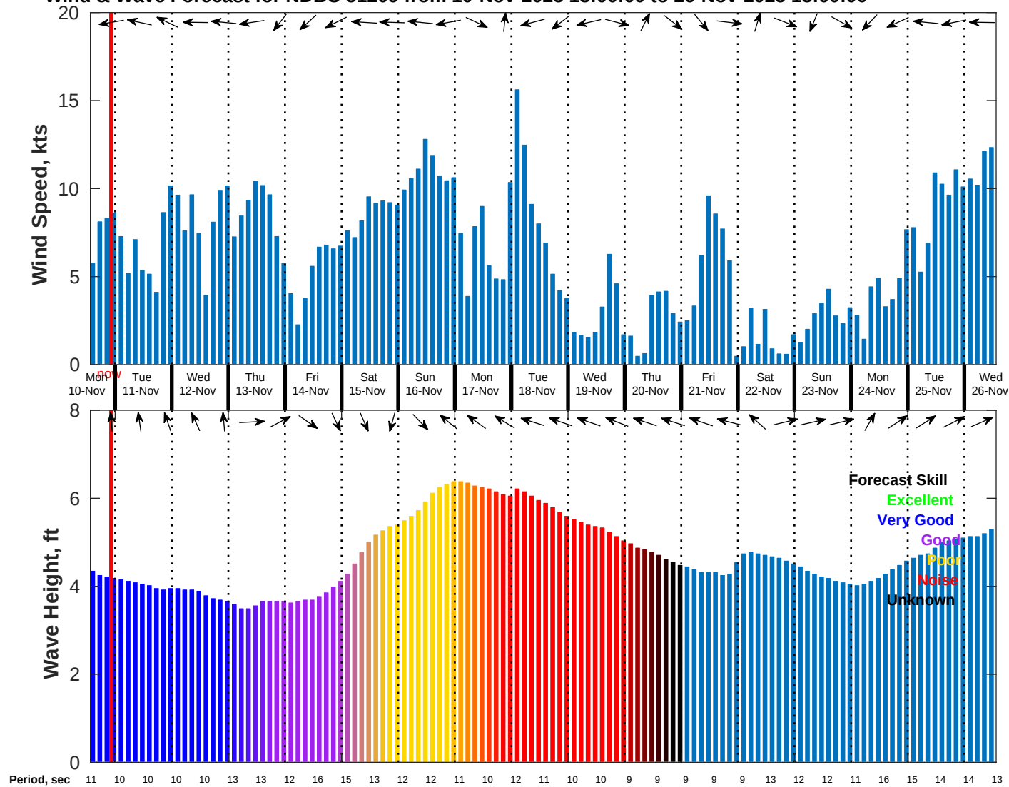
Wind & Wave Forecast for NDBC 51209 from 10-Nov-2025 13:00:00 to 26-Nov-2025 13:00:00
