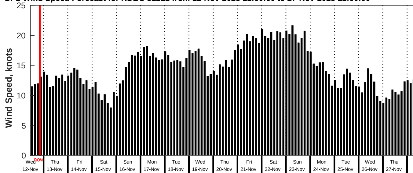
GFS Wind Speed Forecast for NDBC 52211 from 11-Nov-2025 11:00:00 to 27-Nov-2025 11:00:00
