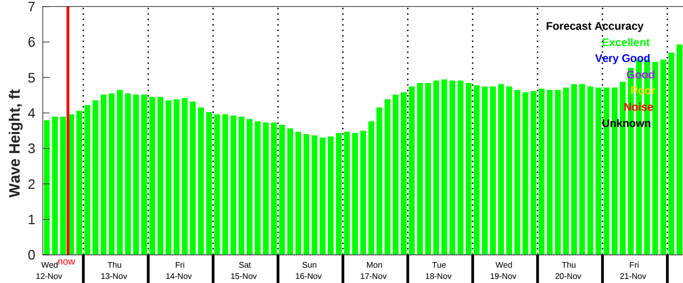
CMEMS Wave Forecast for NDBC 52212 from 11-Nov-2025 09:00:00 to 21-Nov-2025 09:00:00
