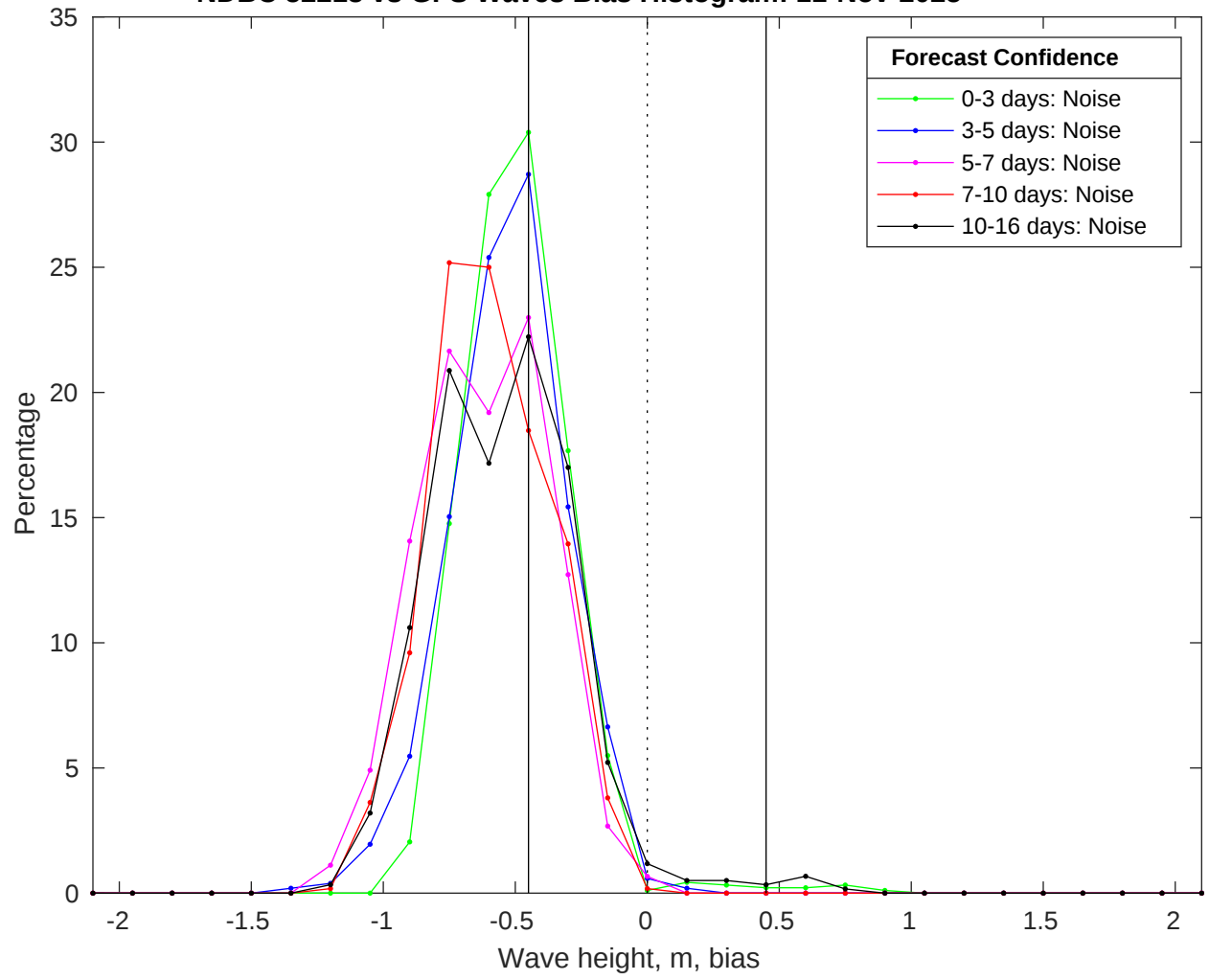
NDBC 52213 vs GFS Waves Bias Histogram: 11-Nov-2025
