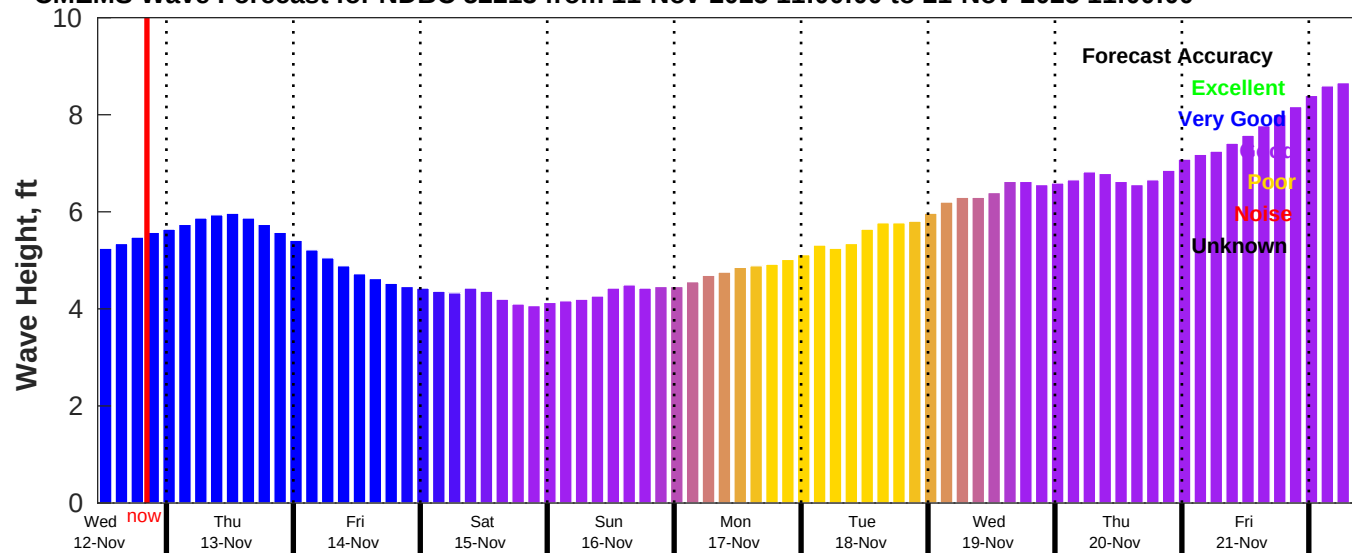
CMEMS Wave Forecast for NDBC 52213 from 11-Nov-2025 11:00:00 to 21-Nov-2025 11:00:00
