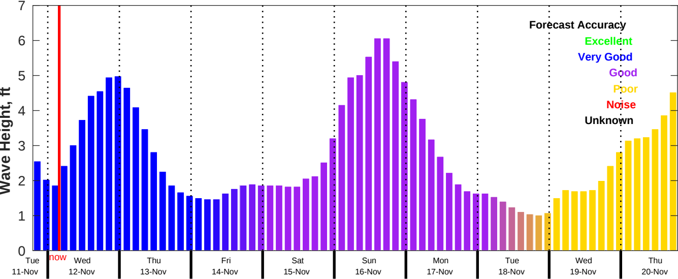
CMEMS Wave Forecast for NDBC 41004 from 11-Nov-2025 19:00:00 to 20-Nov-2025 19:00:00
