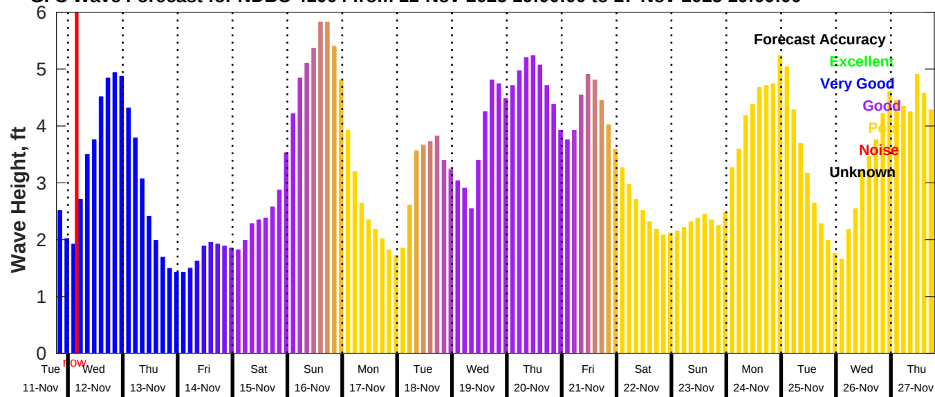
GFS Wave Forecast for NDBC 41004 from 11-Nov-2025 19:00:00 to 27-Nov-2025 19:00:00
