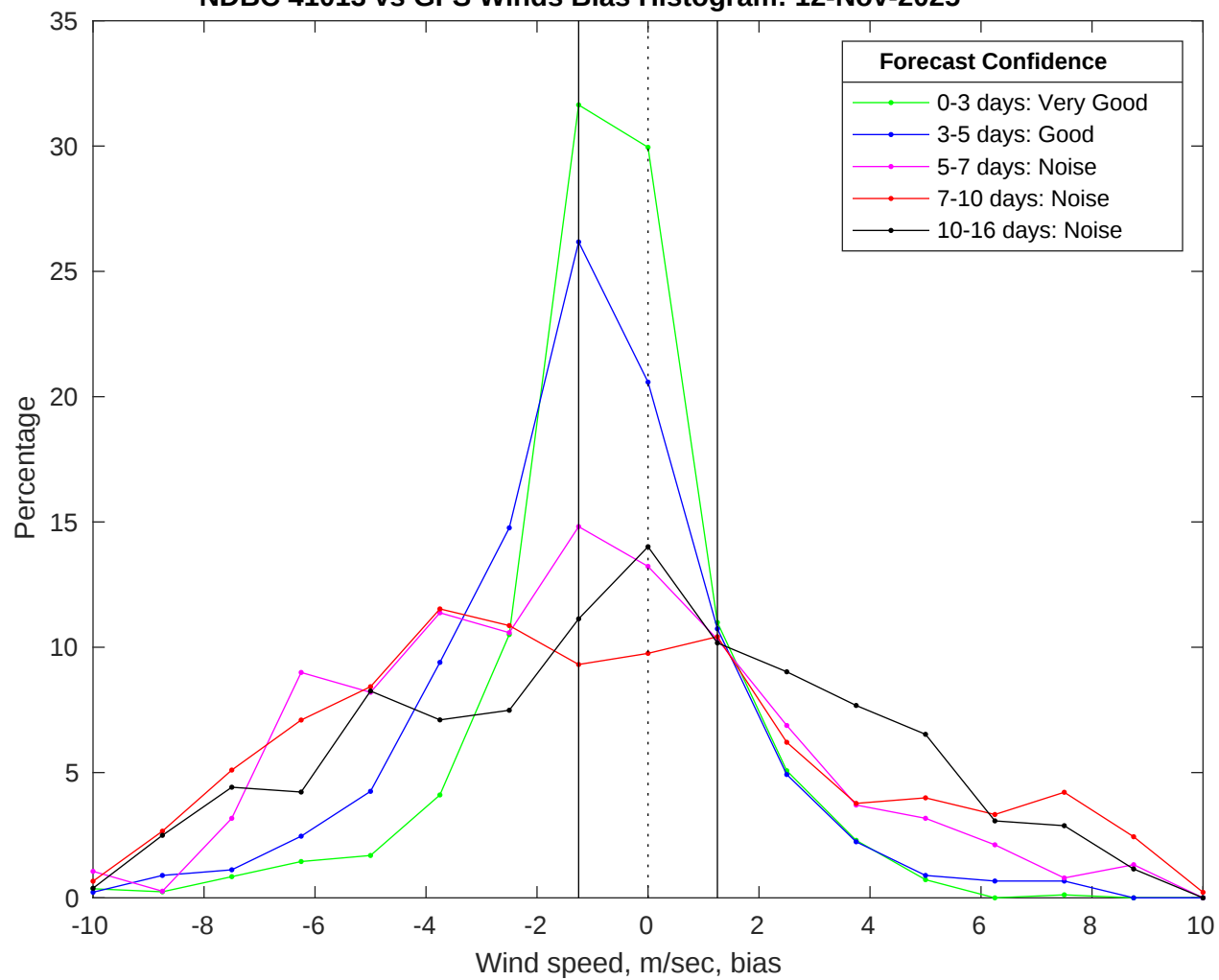
NDBC 41013 vs GFS Winds Bias Histogram: 12-Nov-2025
