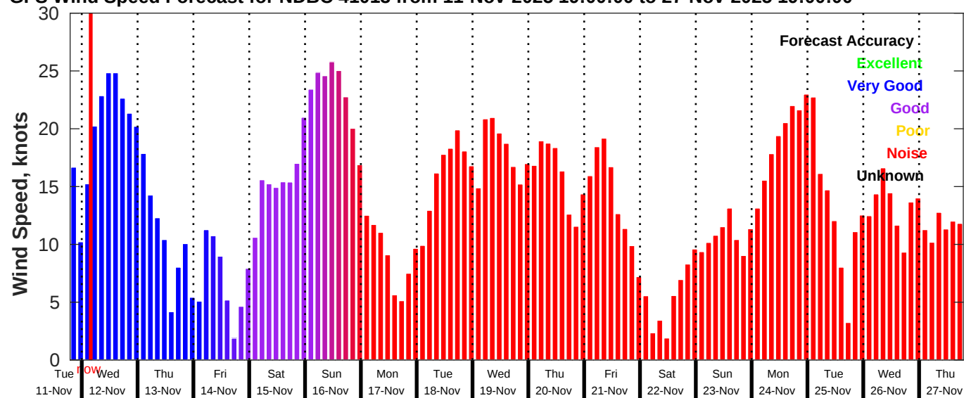
GFS Wind Speed Forecast for NDBC 41013 from 11-Nov-2025 19:00:00 to 27-Nov-2025 19:00:00
