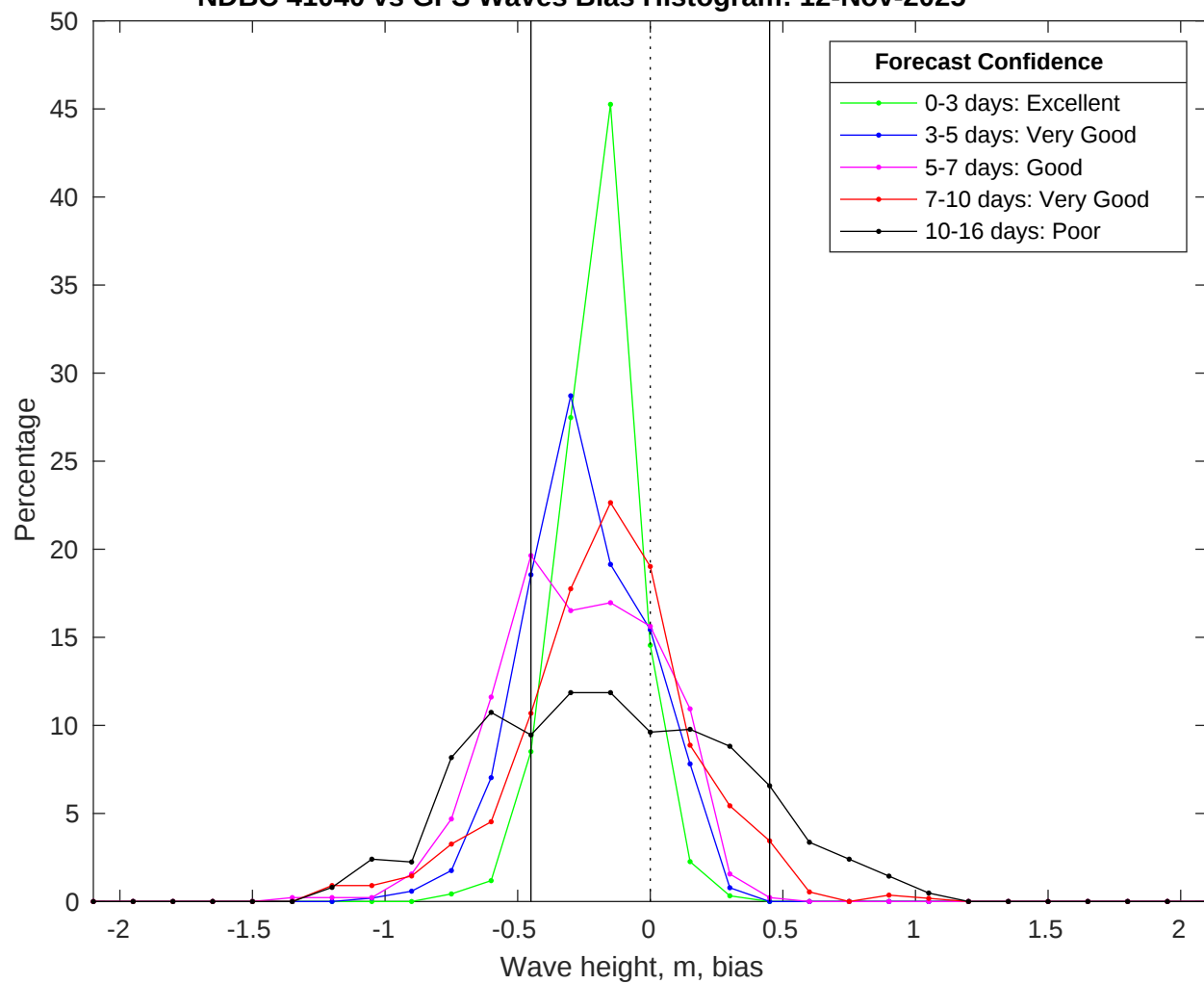
NDBC 41040 vs GFS Waves Bias Histogram: 12-Nov-2025
