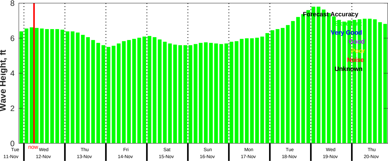
CMEMS Wave Forecast for NDBC 41040 from 11-Nov-2025 21:00:00 to 20-Nov-2025 21:00:00
