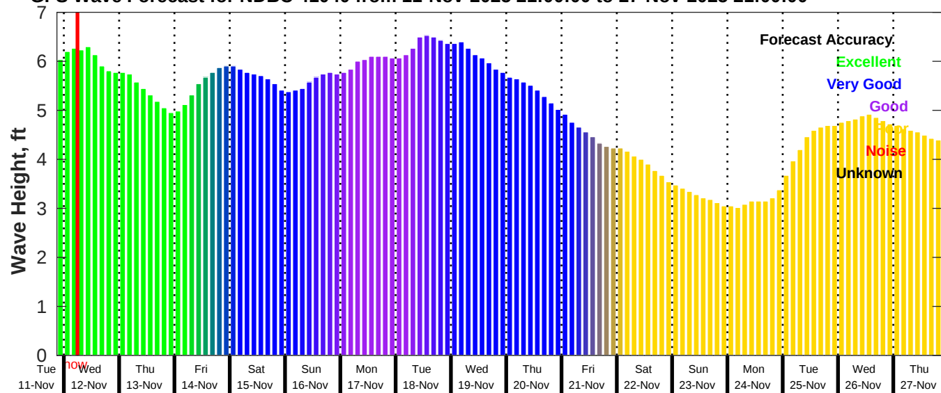
GFS Wave Forecast for NDBC 41040 from 11-Nov-2025 21:00:00 to 27-Nov-2025 21:00:00
