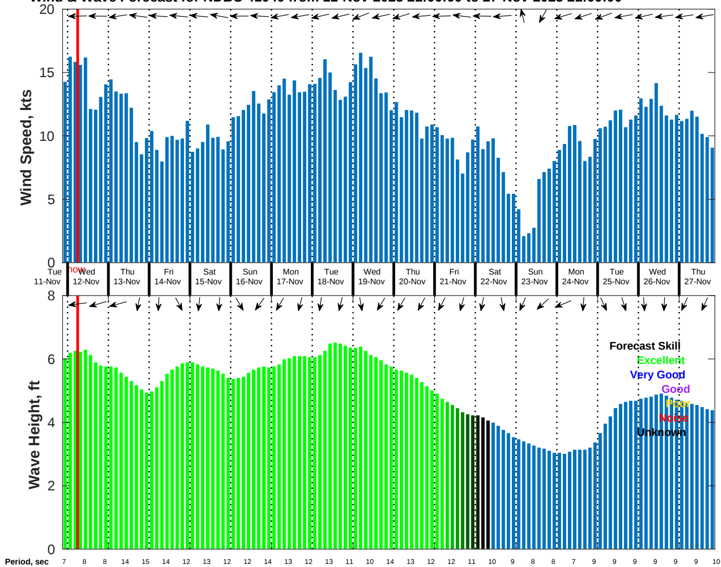
Wind & Wave Forecast for NDBC 41040 from 11-Nov-2025 21:00:00 to 27-Nov-2025 21:00:00
