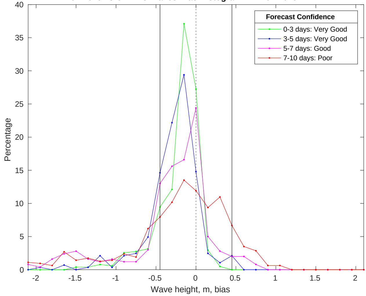
NDBC 42019 vs CMEMS Waves Bias Histogram: 12-Nov-2025
