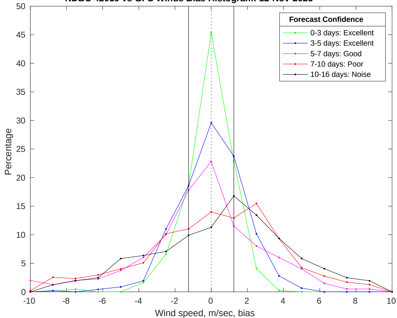
NDBC 42019 vs GFS Winds Bias Histogram: 12-Nov-2025
