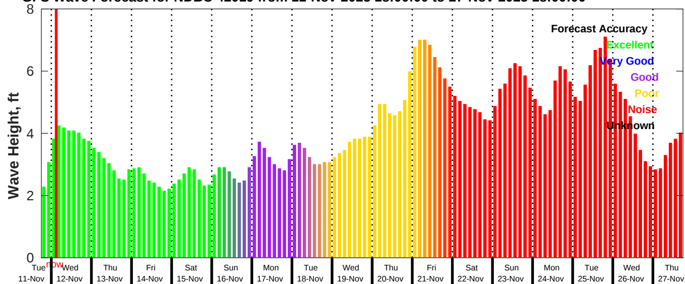
GFS Wave Forecast for NDBC 42019 from 11-Nov-2025 18:00:00 to 27-Nov-2025 18:00:00
