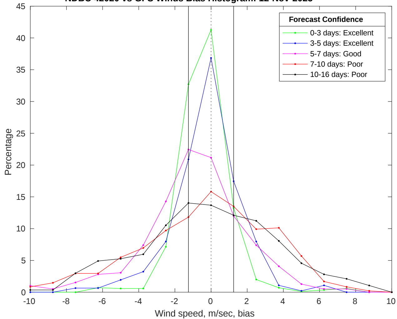
NDBC 42020 vs GFS Winds Bias Histogram: 12-Nov-2025
