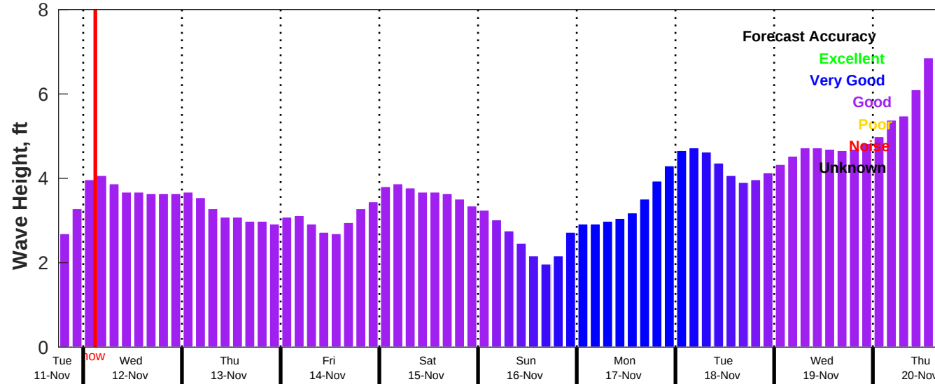
CMEMS Wave Forecast for NDBC 42020 from 11-Nov-2025 18:00:00 to 20-Nov-2025 18:00:00
