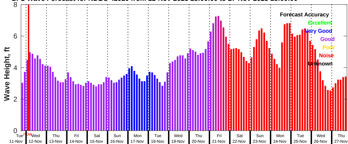
GFS Wave Forecast for NDBC 42020 from 11-Nov-2025 18:00:00 to 27-Nov-2025 18:00:00
