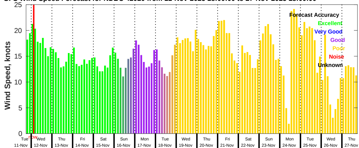
GFS Wind Speed Forecast for NDBC 42020 from 11-Nov-2025 18:00:00 to 27-Nov-2025 18:00:00
