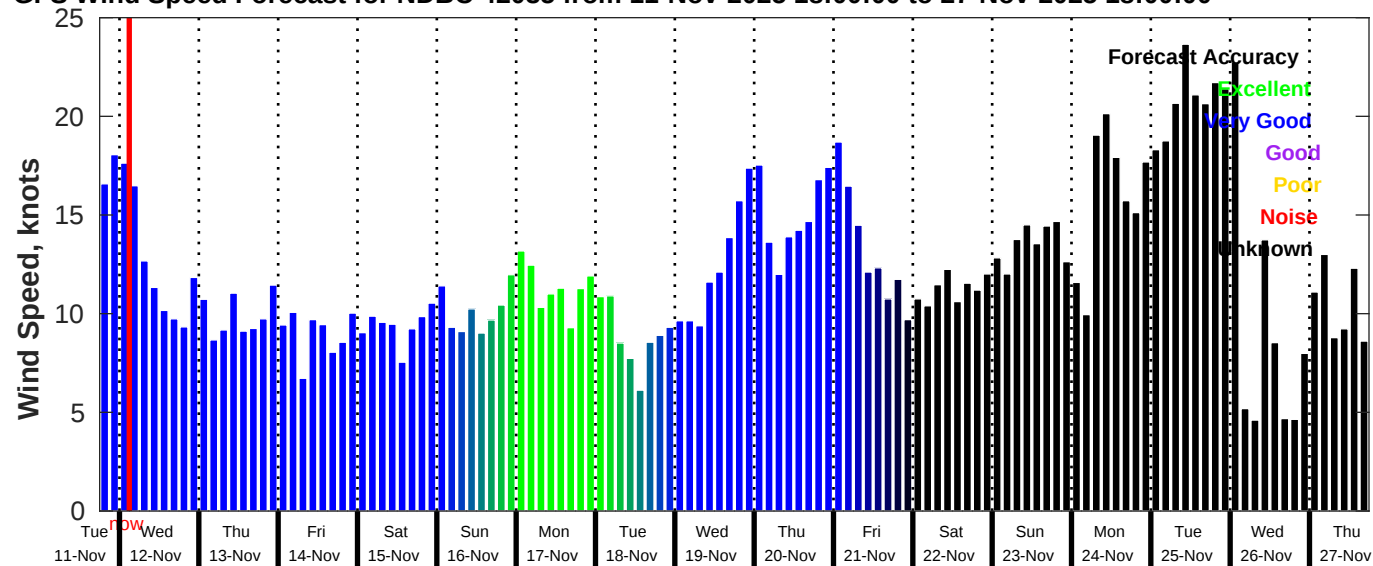
GFS Wind Speed Forecast for NDBC 42035 from 11-Nov-2025 18:00:00 to 27-Nov-2025 18:00:00
