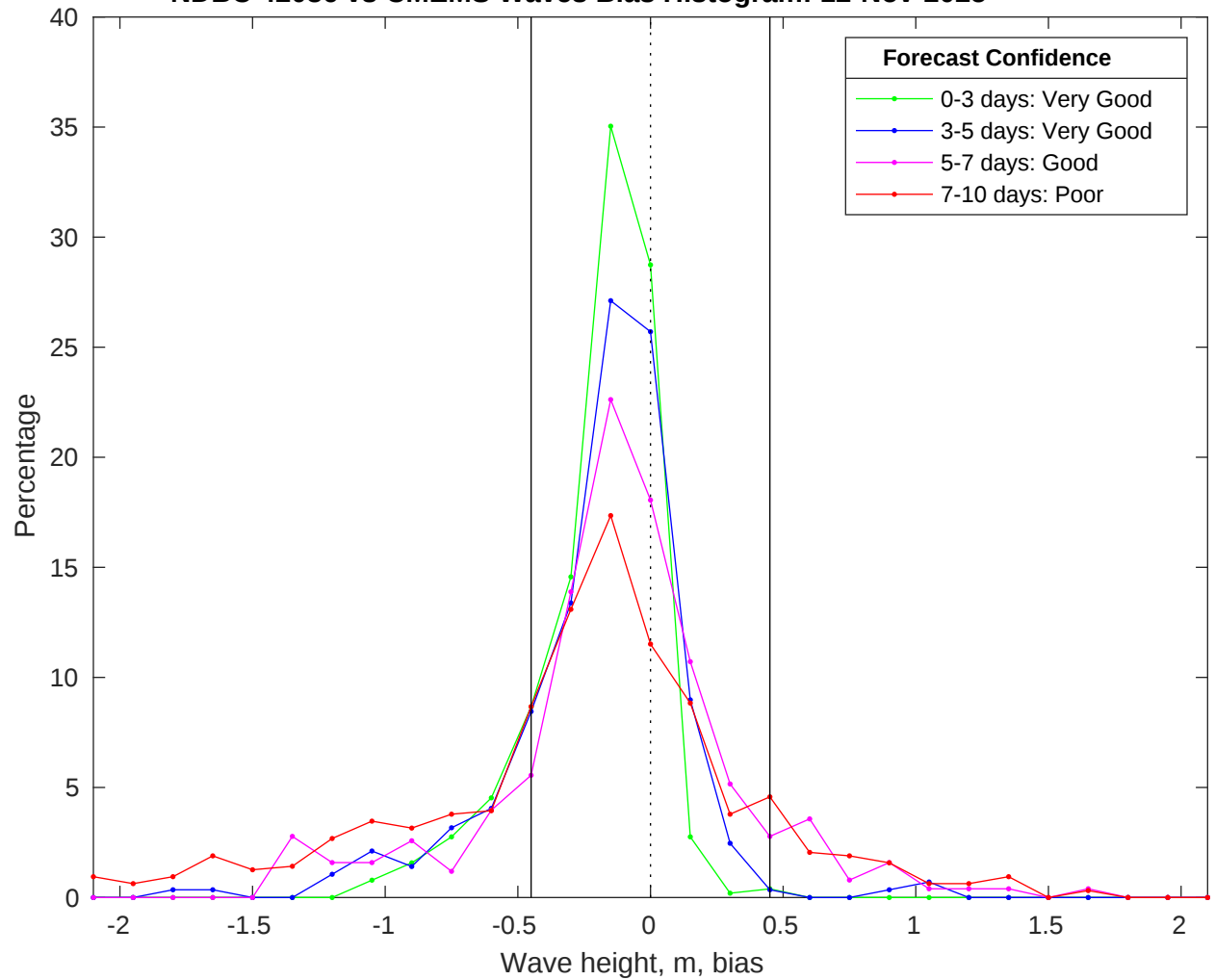
NDBC 42036 vs CMEMS Waves Bias Histogram: 12-Nov-2025
