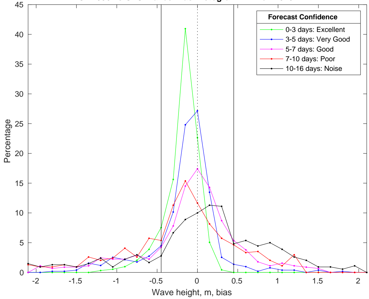
NDBC 42036 vs GFS Waves Bias Histogram: 12-Nov-2025
