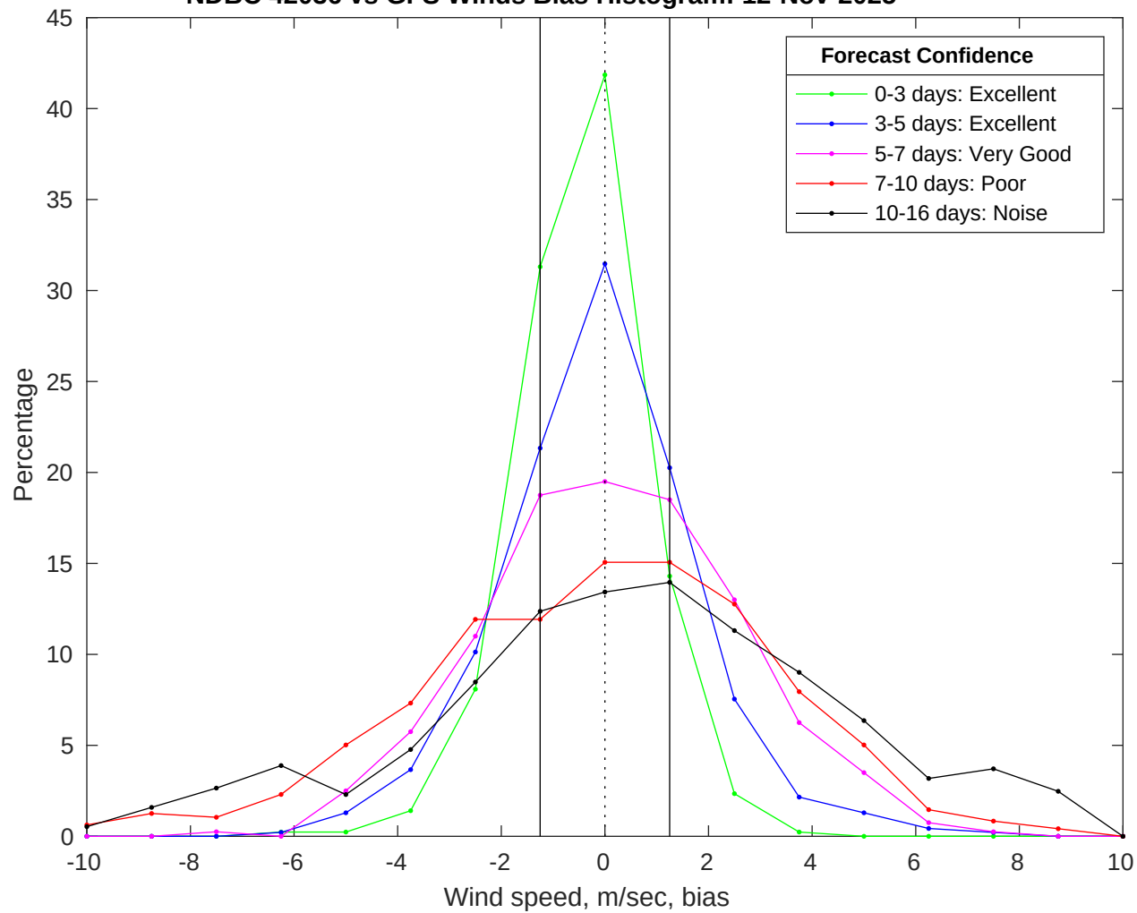
NDBC 42036 vs GFS Winds Bias Histogram: 12-Nov-2025
