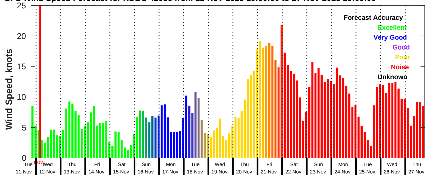
GFS Wind Speed Forecast for NDBC 42036 from 11-Nov-2025 19:00:00 to 27-Nov-2025 19:00:00
